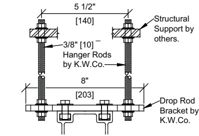
Optional Drop Rod Bracket Mount
