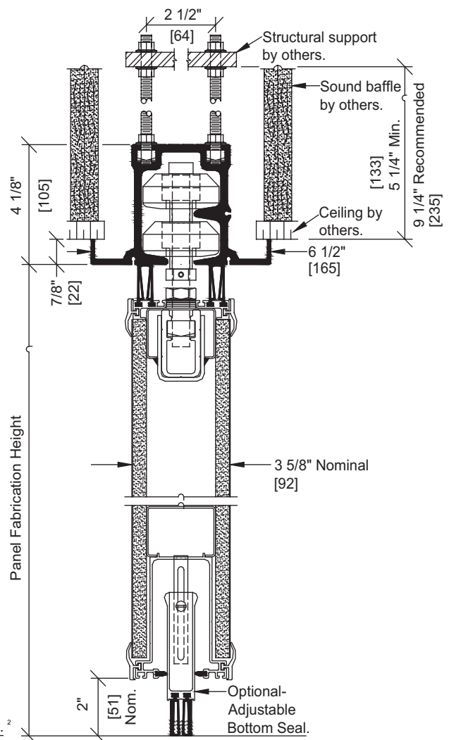
850 Multi-Directional Aluminum Track and Carrier
