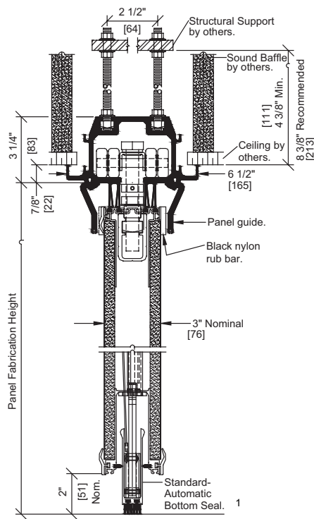
850 Continuously Hinged/Manual Aluminum Track and Carrier
