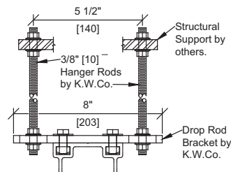
Optional Drop Rod Bracket Mount
