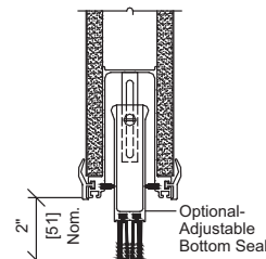
Optional Adjustable Bottom Seal
