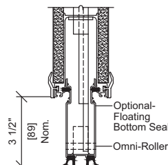
Optional Floating Bottom Seal
