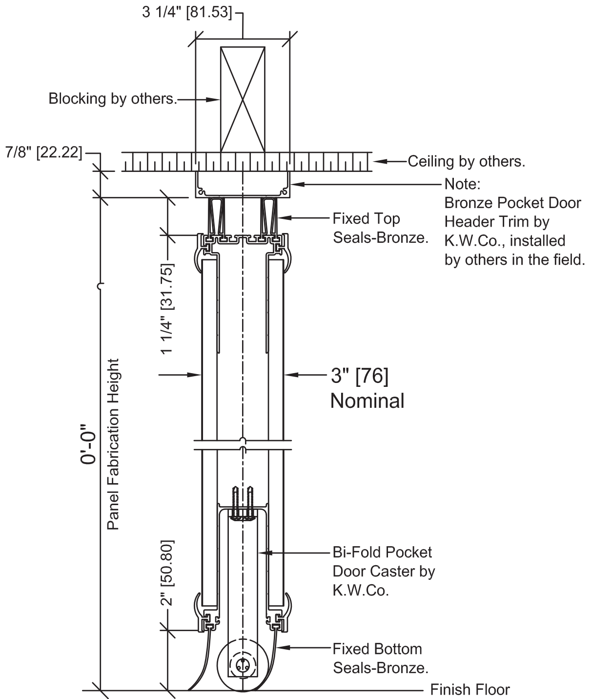
Bi-Fold Pocket Door
