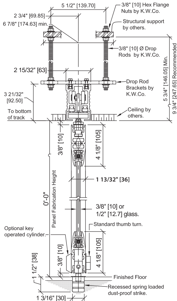
Drop Rod Bracket Mount Variotec Trimmed
