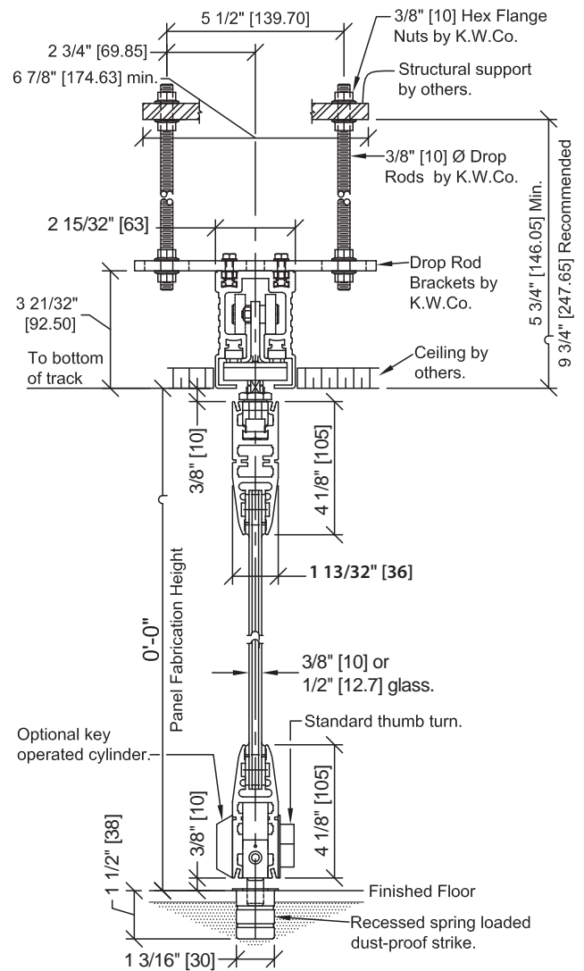
Drop Rod Bracket Mount Variotec Trimless
