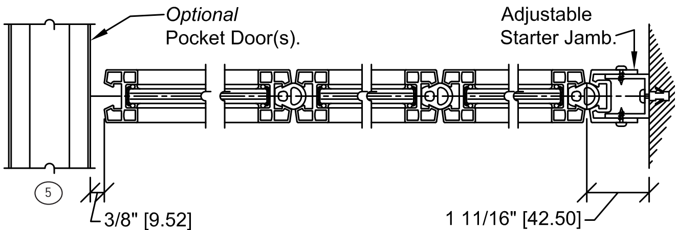
HORIZONTAL DETAIL - KWV-Tec TRIMMED
