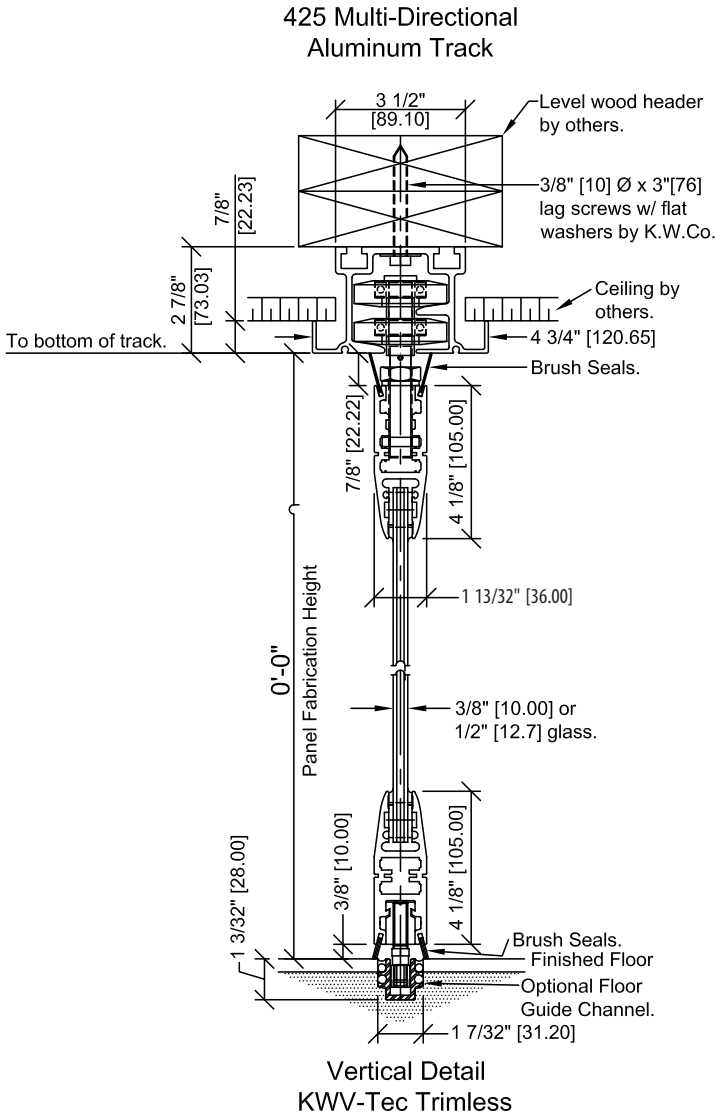
Direct Mount with Floor Guide Channel KWV-Tec Trimless
