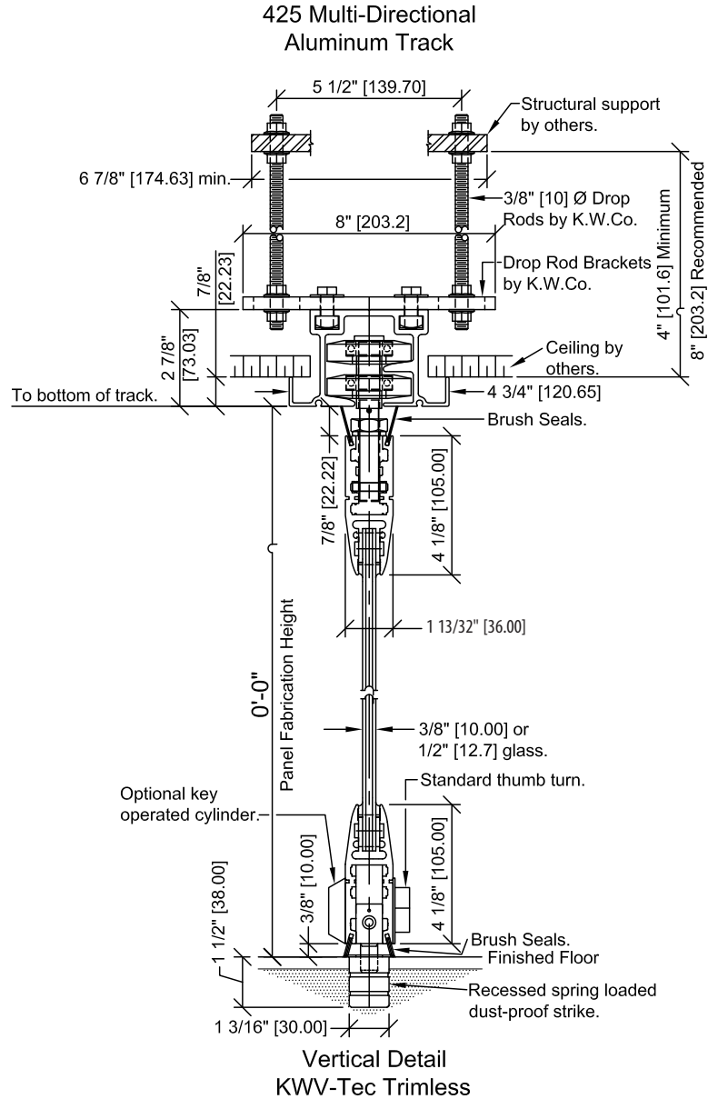
Drop Rod Bracket Mount KWV-Tec Trimless
