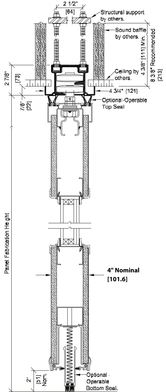
425 Multi-Directional Aluminum Track and Carrier
