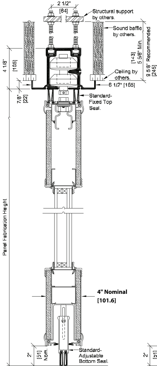
850 Multi-Directional Aluminum Track and Carrier
